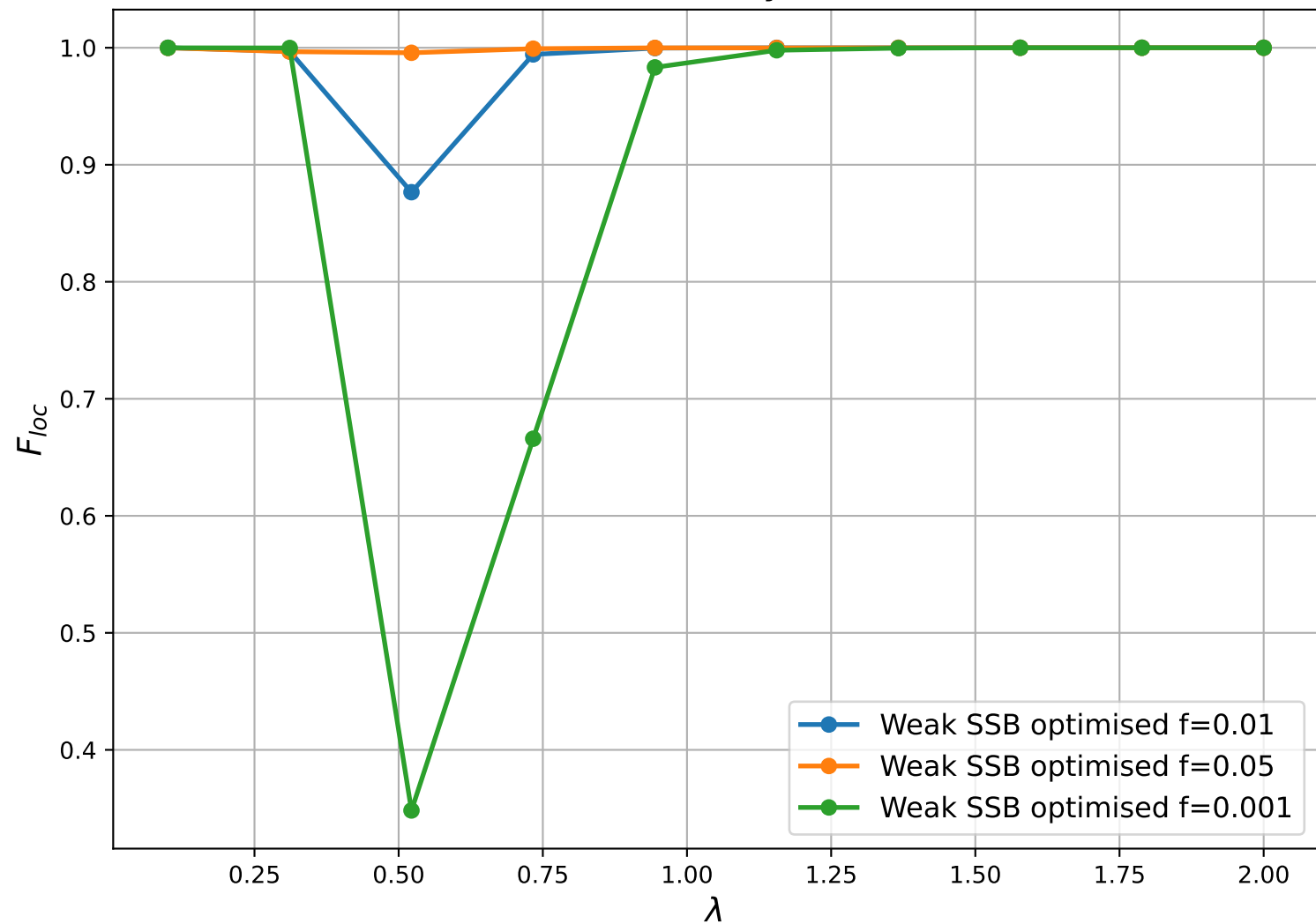
VQE Fidelity vs \lambda
